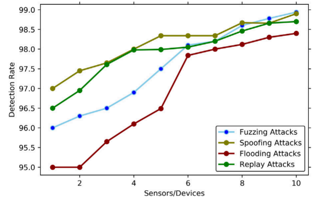
Fig. 6. Detection rates of different types of cyber-attacks.
