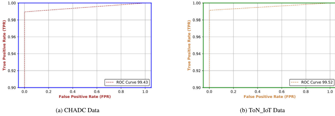
Fig. 4. AUC comparison of proposed trust framework using both data.
